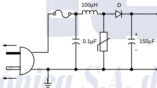
Typical Power Supply Circuit
