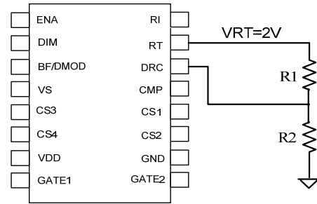
Figure 7 Use DRC PIN to set Dimming Range
