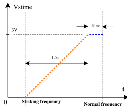
Figure 3 Striking mode control
