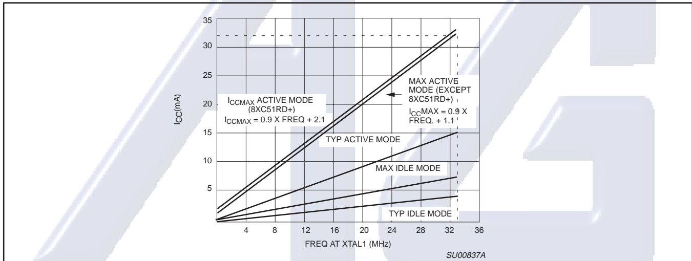
Figure 21. I_{CC} vs. FREQ
