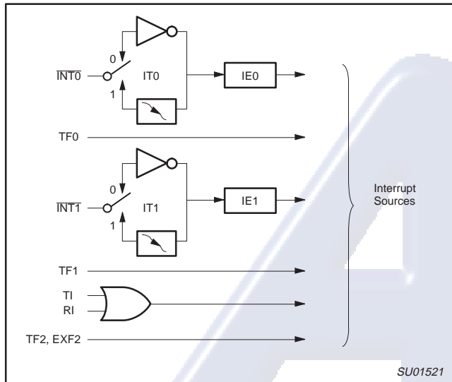
Figure 21. Interrupt Sources
