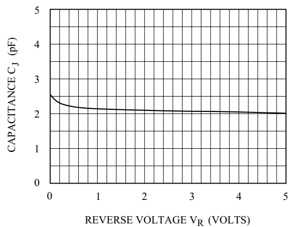
C_J - V_R
