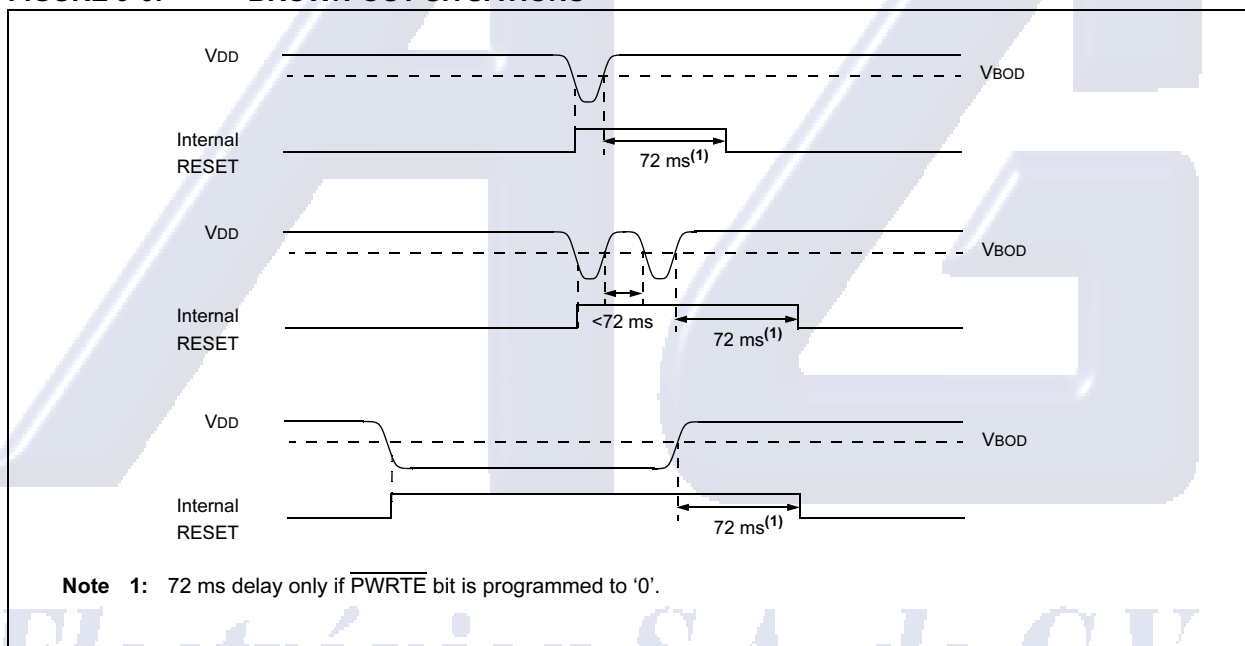
FIGURE 9-6: BROWN-OUT SITUATIONS
