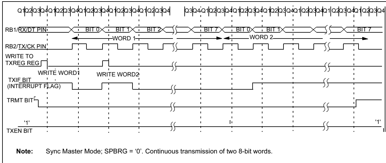
FIGURE 12-12: SYNCHRONOUS TRANSMISSION
