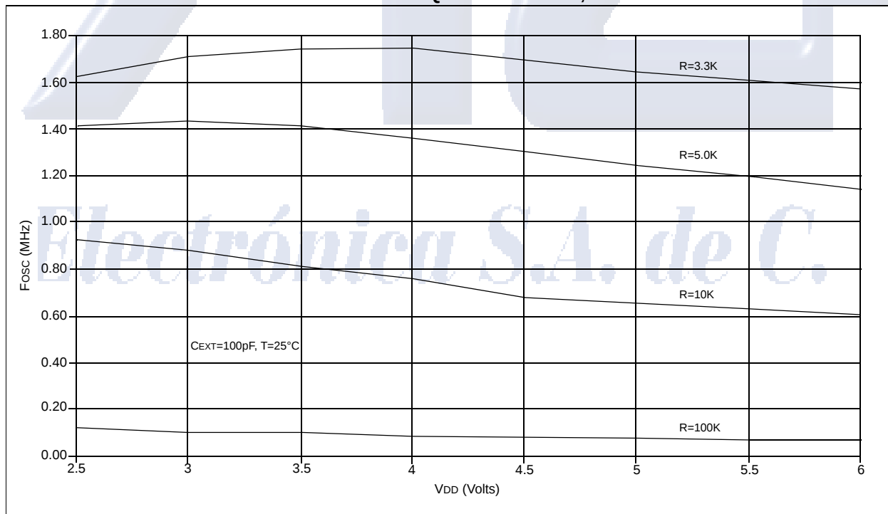
FIGURE 14-3: TYPICAL RC OSCILLATOR FREQUENCY vs. V_{DD} , C_{EXT} = 100\text{ pF}
