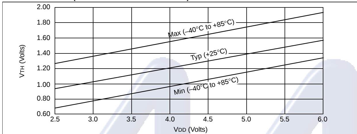
FIGURE 11-10: V_{IH} , V_{IL} OF MCLR, T0CKI AND OSC1 (IN RC MODE) vs. V_{DD}
