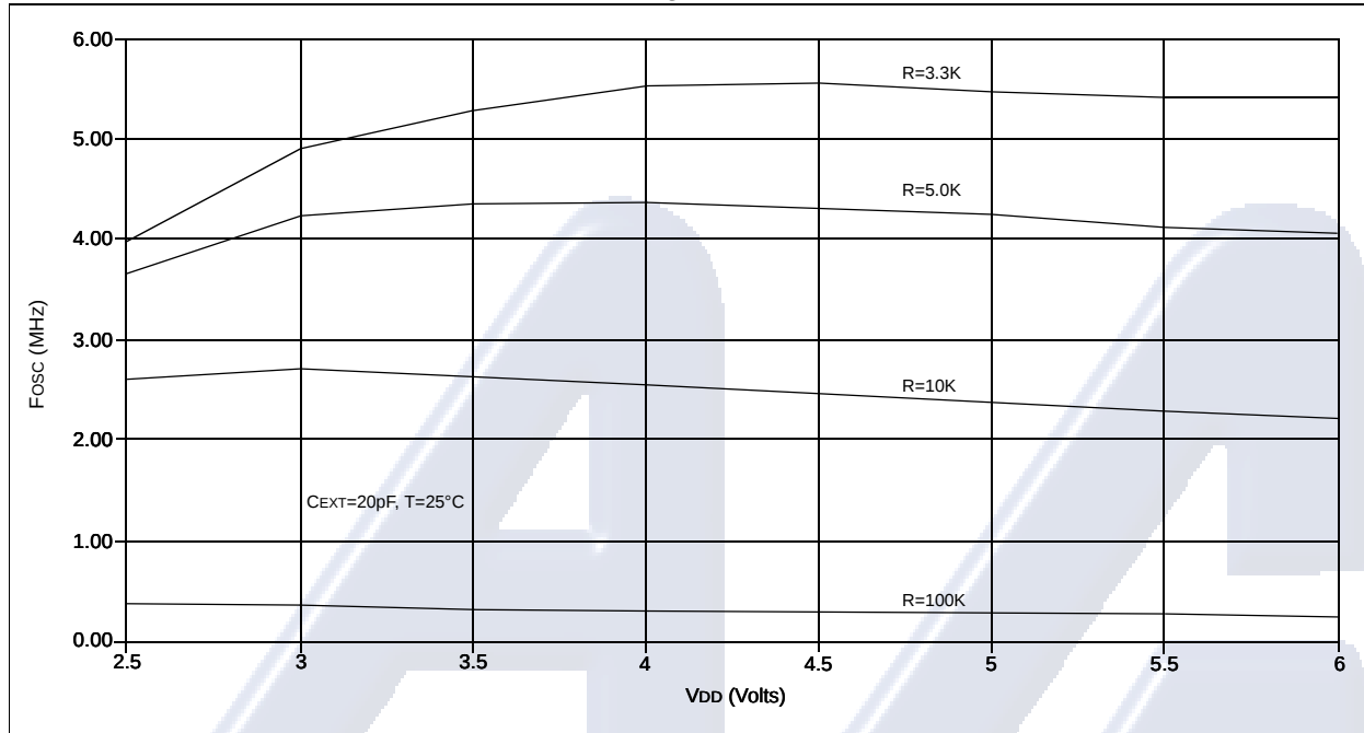
FIGURE 14-2: TYPICAL RC OSCILLATOR FREQUENCY vs. V_{DD} , C_{EXT} = 20\text{ pF}
