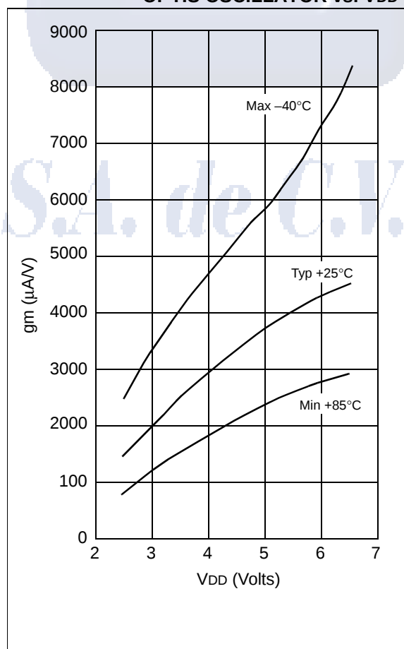
FIGURE 11-16: TRANSCONDUCTANCE ( g_m ) OF HS OSCILLATOR vs. V_{DD}
