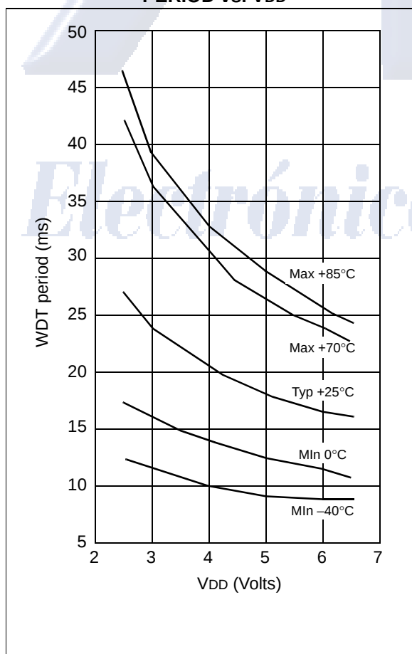
FIGURE 11-15: WDT TIMER TIME-OUT PERIOD vs. V_{DD}
