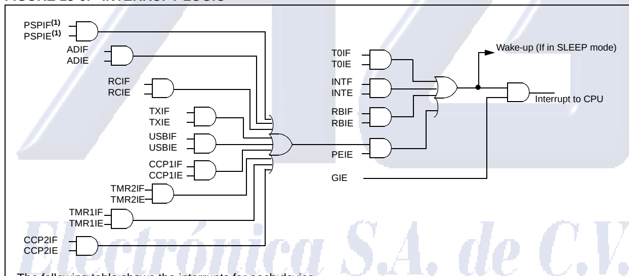
FIGURE 13-6: INTERRUPT LOGIC
