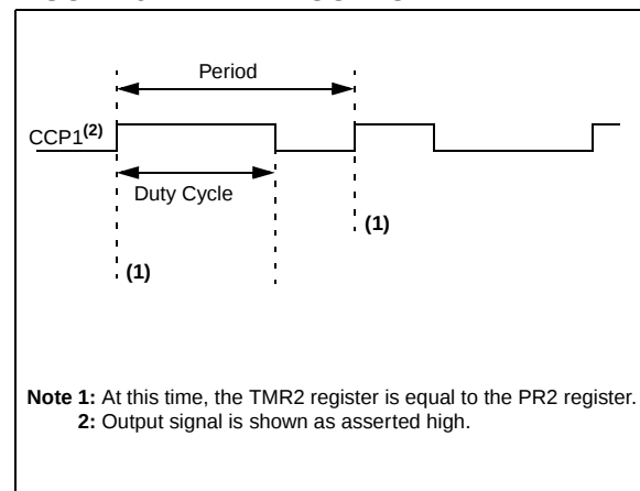
FIGURE 9-4: PWM OUTPUT
