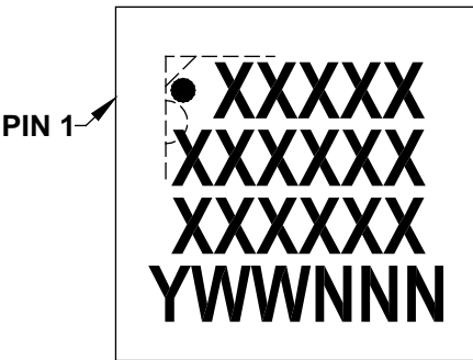
16-Lead QFN (4x4x0.9 mm) 16-Lead UQFN (4x4x0.5 mm)
