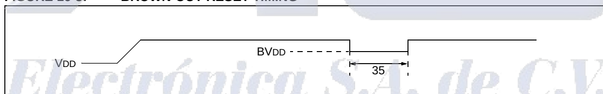
FIGURE 16-8: BROWN-OUT RESET TIMING
