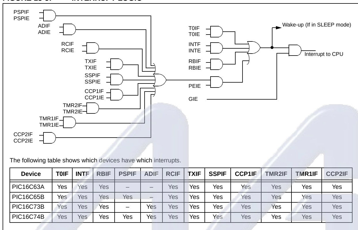
FIGURE 13-5: INTERRUPT LOGIC
