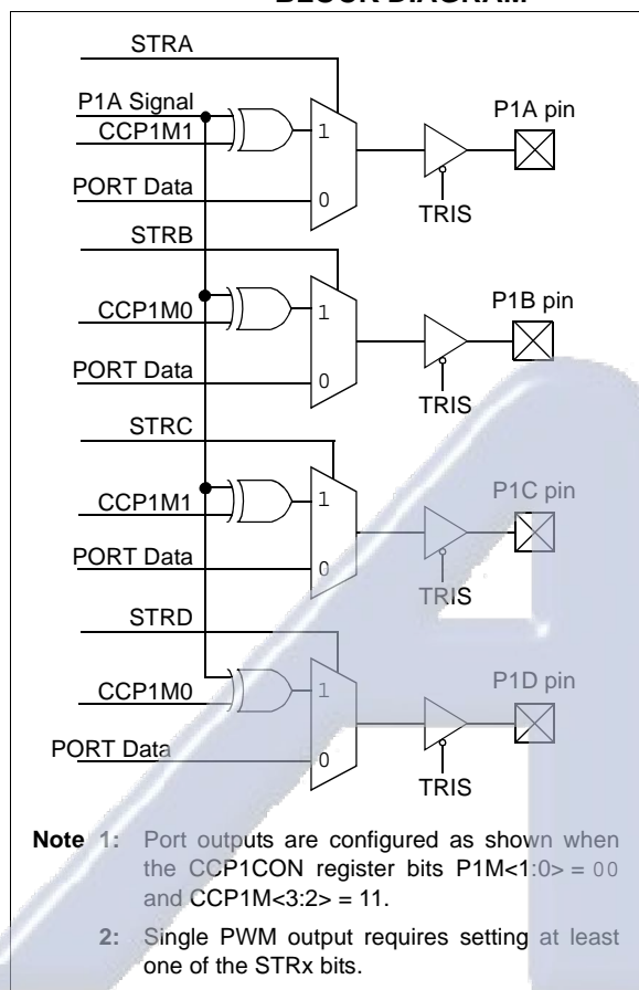
FIGURE 11-19: SIMPLIFIED STEERING BLOCK DIAGRAM
