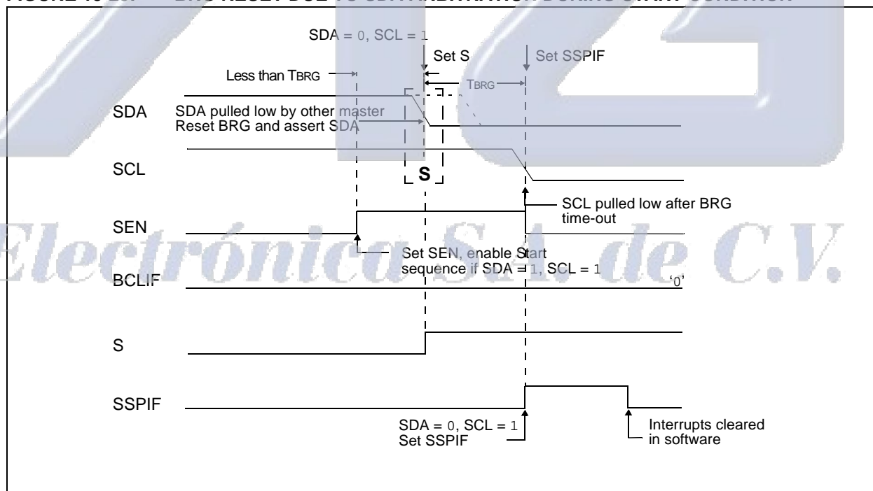
FIGURE 13-23: BRG RESET DUE TO SDA ARBITRATION DURING START CONDITION
