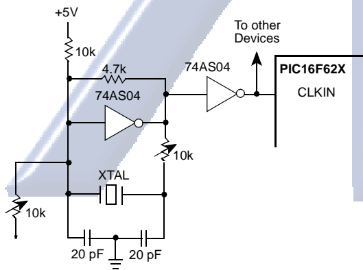
FIGURE 14-4: EXTERNAL PARALLEL RESONANT CRYSTAL OSCILLATOR CIRCUIT
