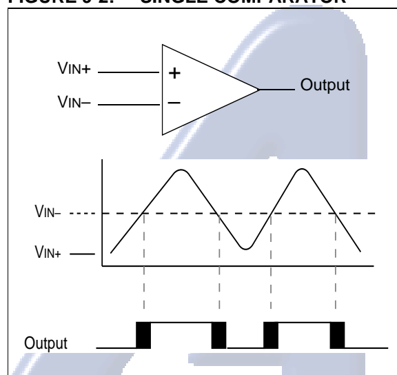
FIGURE 9-2: SINGLE COMPARATOR
