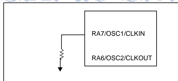
FIGURE 14-7: EXTERNAL RESISTOR
