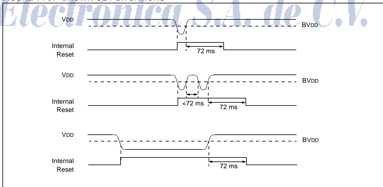
FIGURE 14-9: BROWN-OUT SITUATIONS
