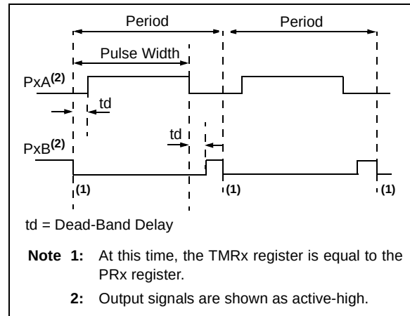
FIGURE 14-8: EXAMPLE OF HALF-BRIDGE PWM OUTPUT
