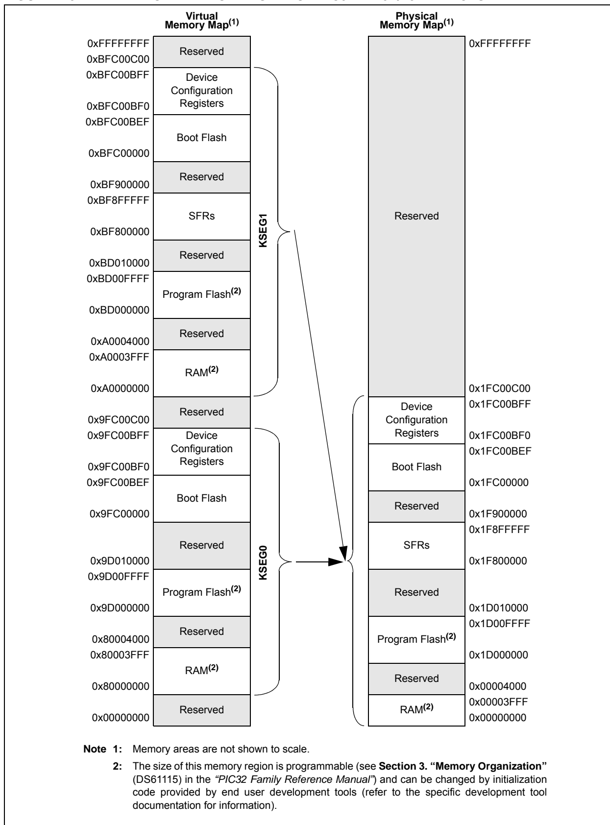
FIGURE 4-3: MEMORY MAP ON RESET FOR PIC32MX13X/23X DEVICES
