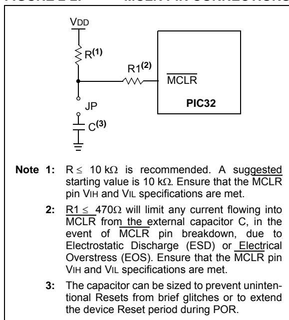
FIGURE 2-2: \overline{\text{MCLR}} PIN CONNECTIONS
