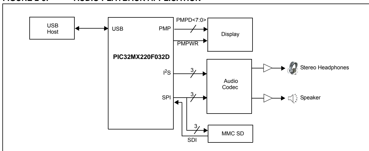
FIGURE 2-5: AUDIO PLAYBACK APPLICATION
