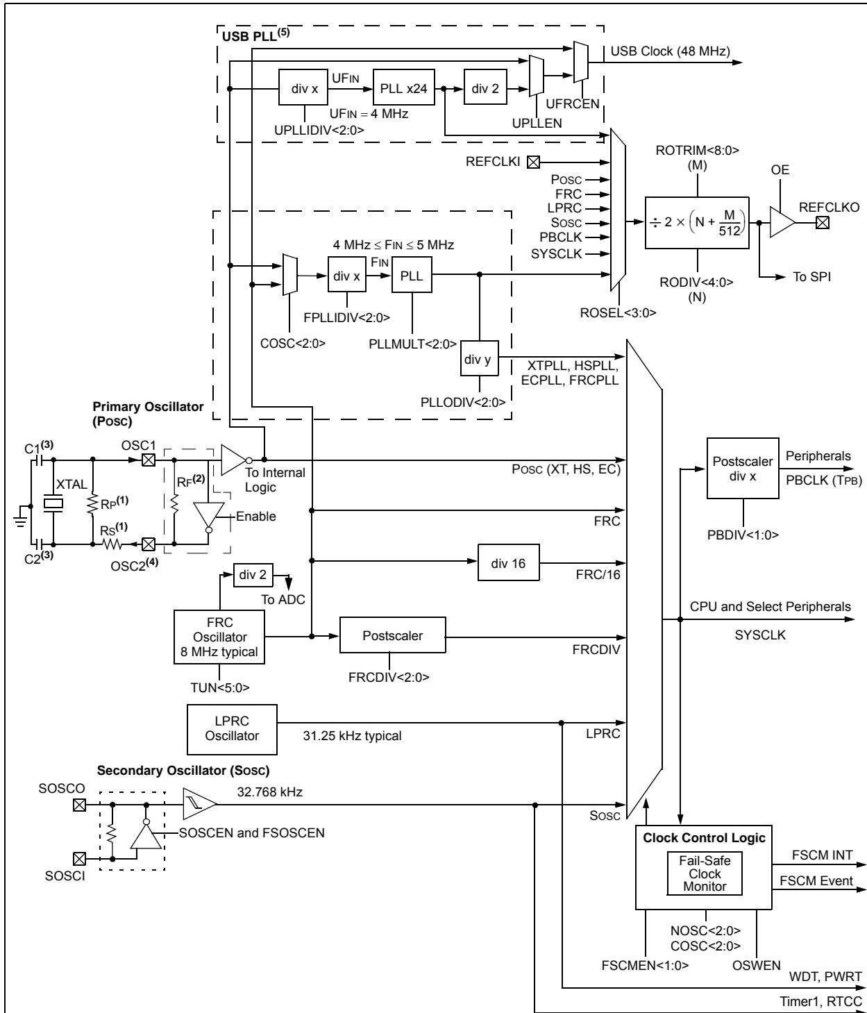
FIGURE 8-1: OSCILLATOR DIAGRAM
