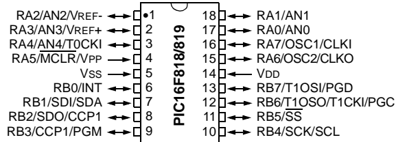
18-Pin PDIP, SOIC
