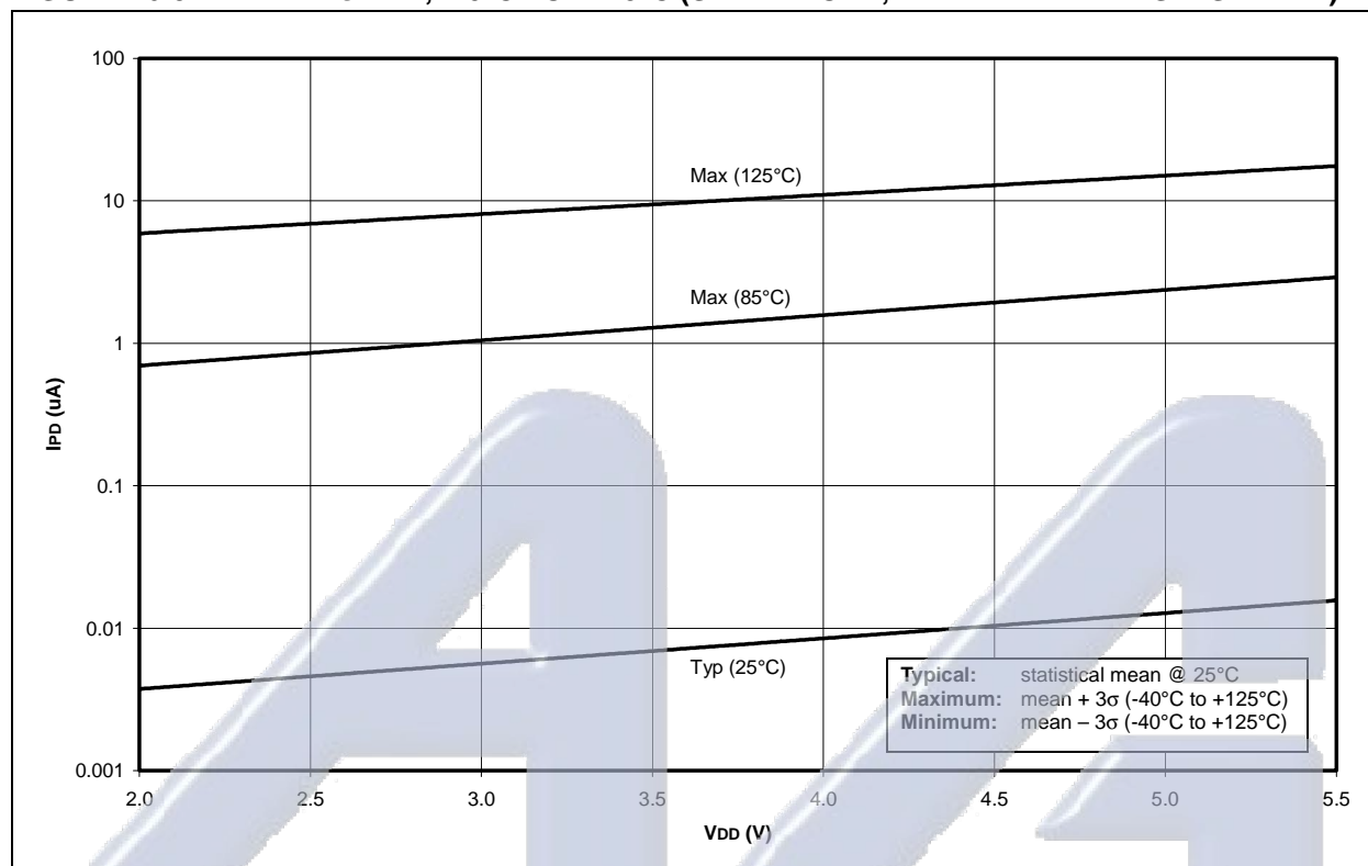
FIGURE 16-9: I_{PD} vs. V_{DD} , -40^{\circ}\text{C} TO +125^{\circ}\text{C} (SLEEP MODE, ALL PERIPHERALS DISABLED)
