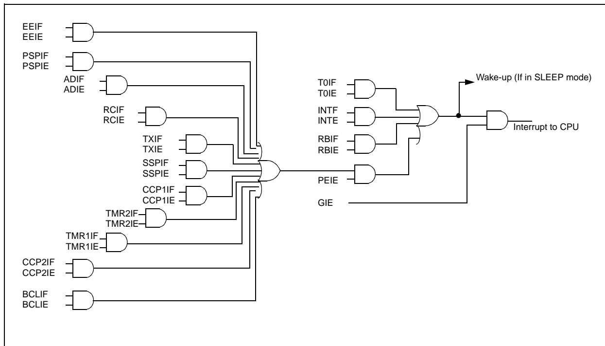
FIGURE 12-9: INTERRUPT LOGIC
