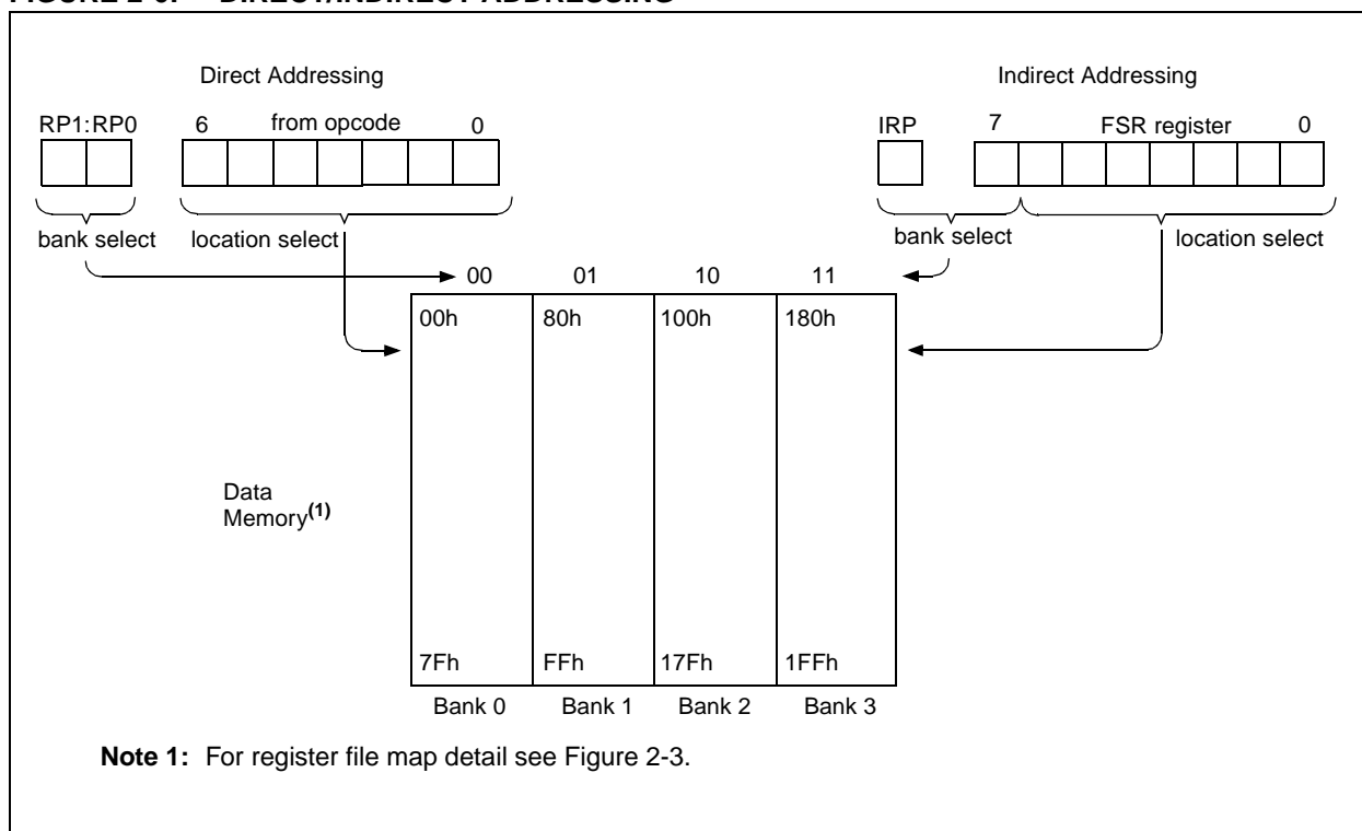
FIGURE 2-6: DIRECT/INDIRECT ADDRESSING
