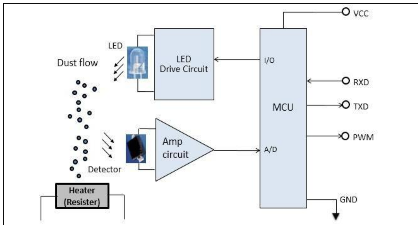
Fig 1 Interior configuration
