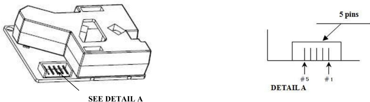
Fig 2 Connector Dimensions
