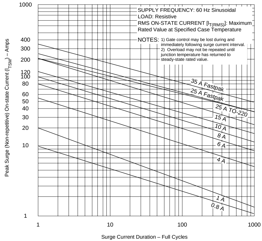
Figure E2.13 Peak Surge Current versus Surge Current Duration
