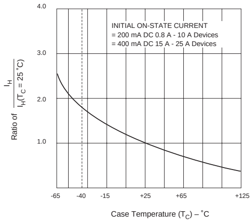
Figure E2.14 Normalized DC Holding Current versus Case Temperature
