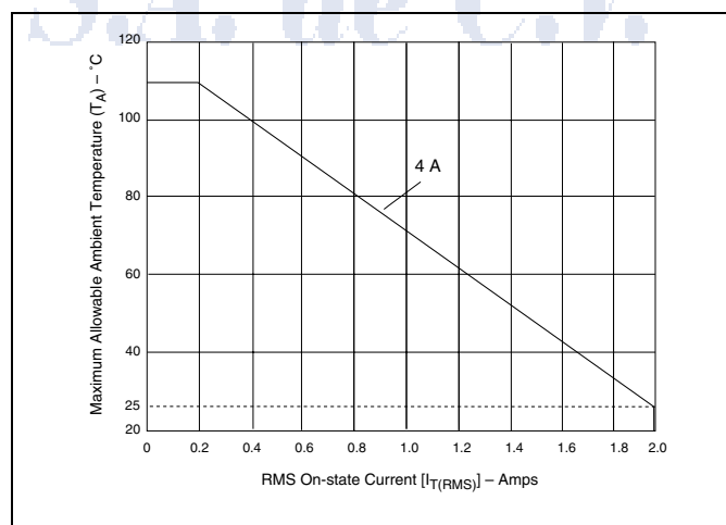
Figure E3.6 Maximum Allowable Ambient Temperature versus On-state Current
