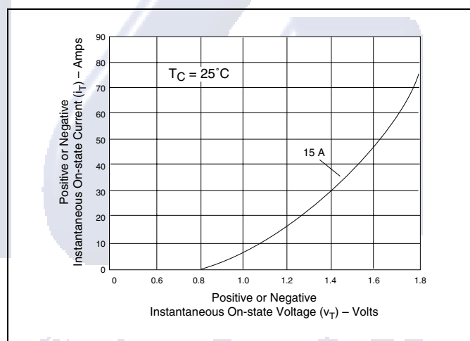
Figure E3.5 On-state Current versus On-state Voltage (Typical) (15 A)
