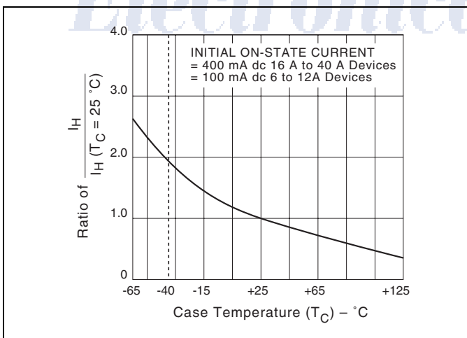
Figure E4.9 Normalized DC Holding Current versus Case Temperature
