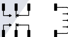
DPDT, 2 Form "C"
