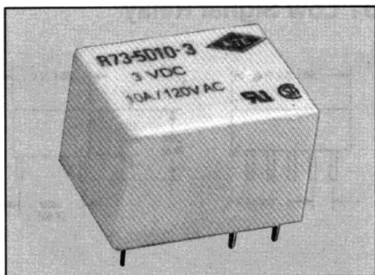
SPST-NO, 1 Form "A"
