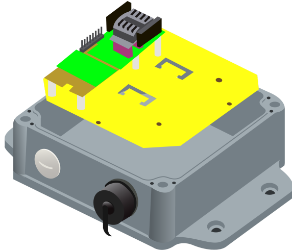
Figure 1: WisBlock RAKBox-B4 Enclosure Top View
