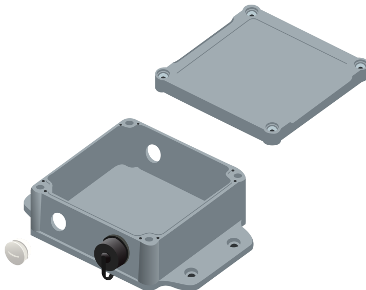
Figure 2: RAKBox-B4 Enclosure Overview
