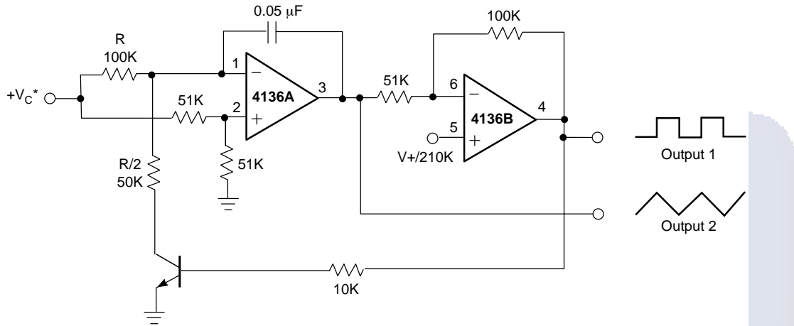
Figure 30. Voltage Control Oscillator (VCO)
