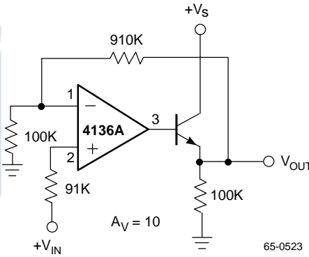
Figure 22. Power Amplifier
