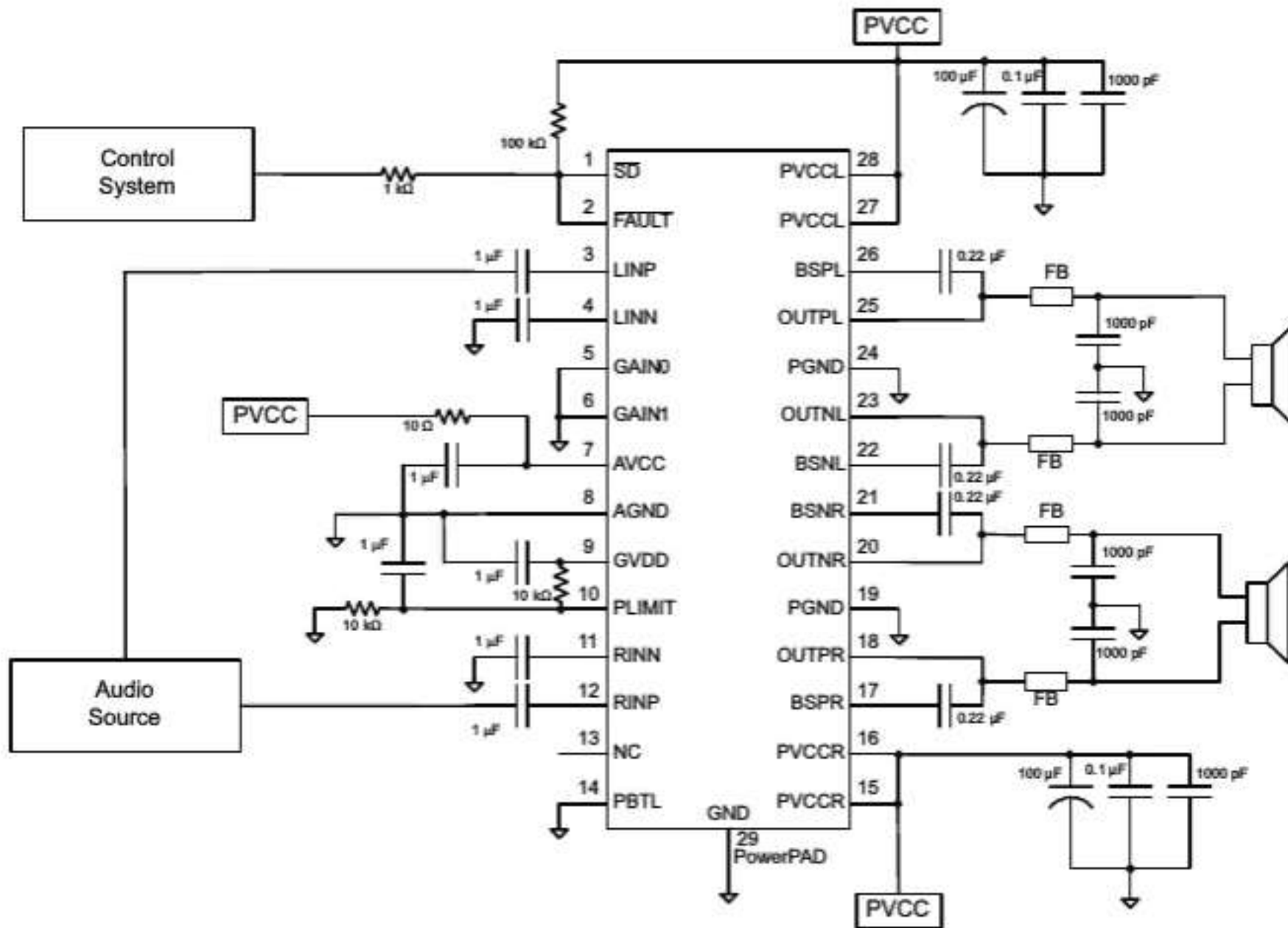
Stereo Class-D Amplifier with BTL Output and Single-Ended Inputs
