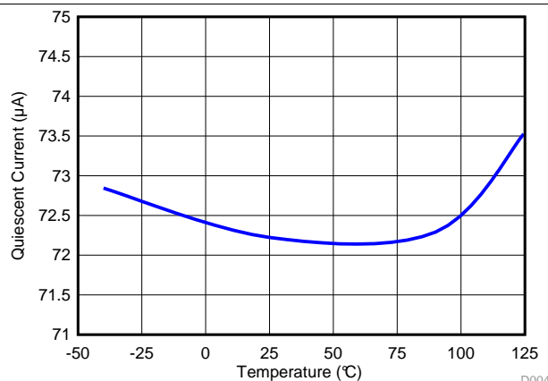
Figure 1. Temperature Drift
