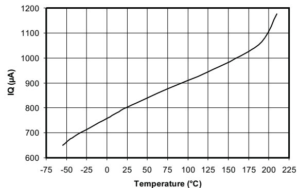
Figure 11. Quiescent Current vs Temperature
