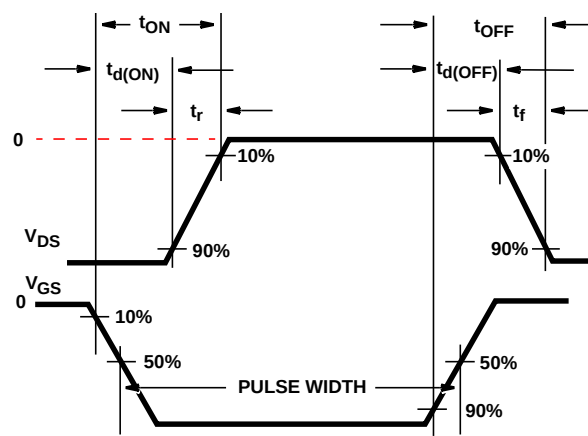
FIGURE 17. RESISTIVE SWITCHING WAVEFORMS
