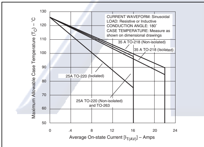
Figure E6.14 Maximum Allowable Case Temperature versus Average On-state Current (25 A and 35 A)
