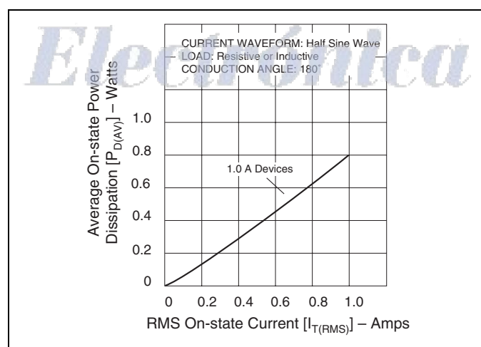
Figure E6.24 Power Dissipation (Typical) versus RMS On-state Current (1 A)
