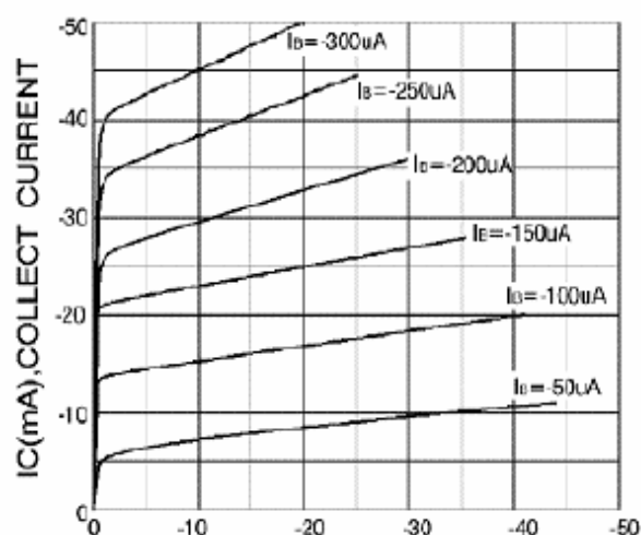
Static Characteristic
