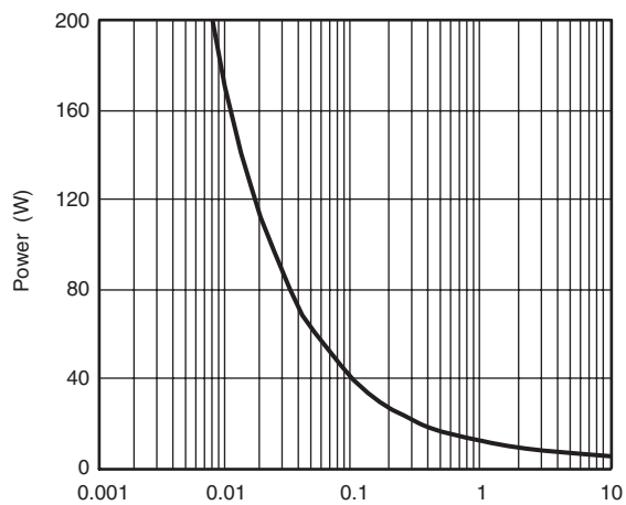
Time (s) Single Pulse Power, Junction-to-Ambient
