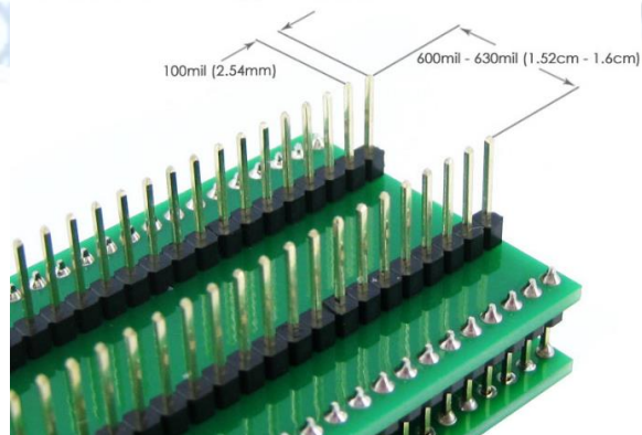
DIP Pin Header Dimensions (For Reference)
