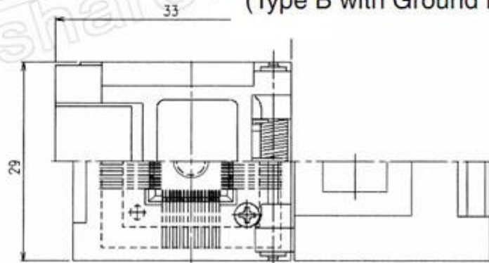
Type BT (Type B with Ground Pin)
