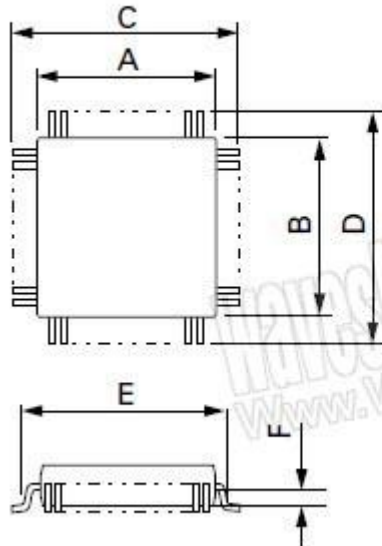
Outline IC Body Dimensions
