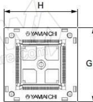
Outline Open Top Socket Dimensions
