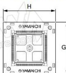
Outline Open Top Socket Dimensions
