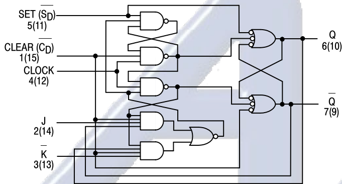
LOGIC DIAGRAM
