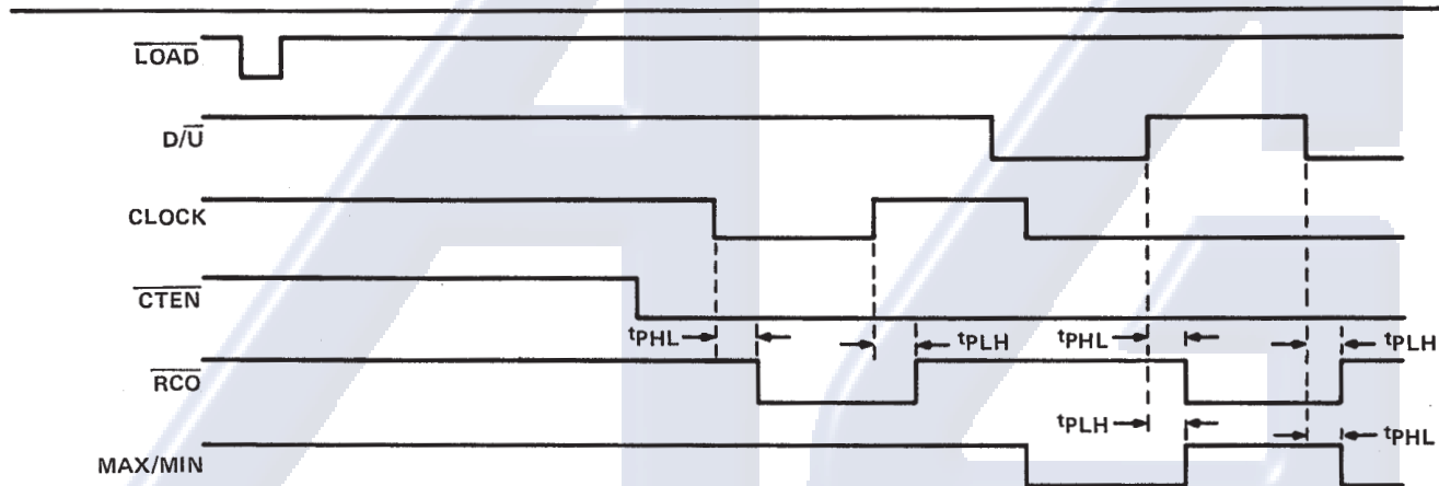
FIGURE 4—LOAD TO OUTPUT AND DATA TO OUTPUT
