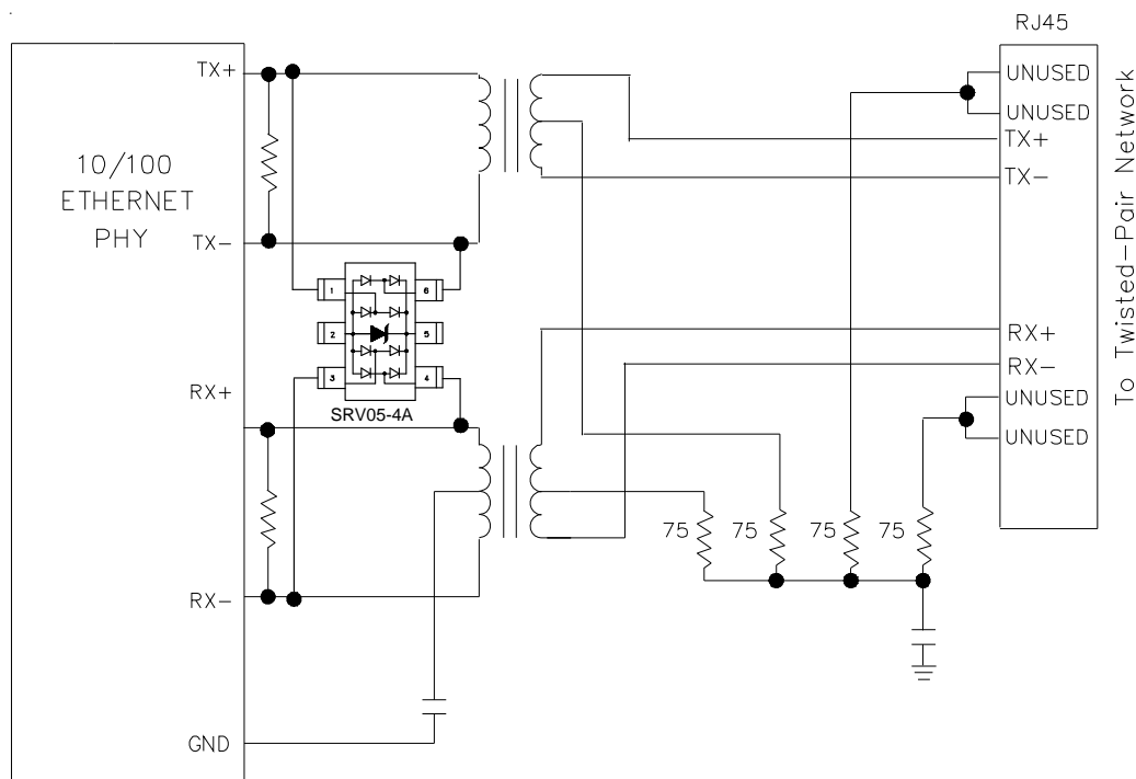
Figure 9 - 10/100 Ethernet Differential and Common Mode Protection
