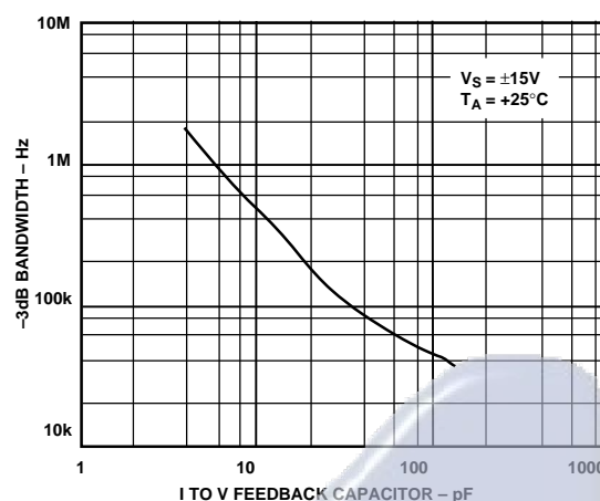
Figure 17. -3 dB Bandwidth vs. I-to-V Feedback Capacitor
