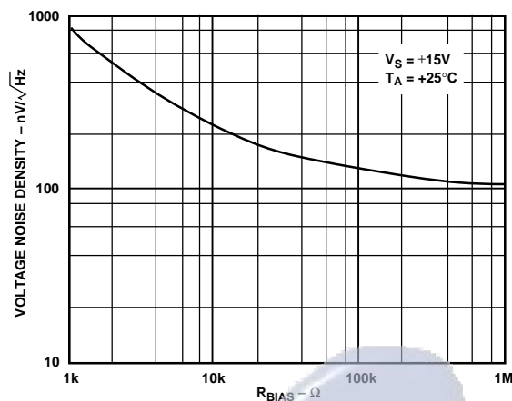
Figure 11. Voltage Noise Density vs. R_{BIAS}
