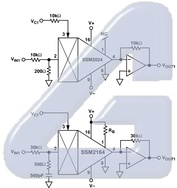
Figure 28. Upgrading SSM2024 Sockets with SSM2164
