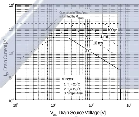
Figure 9-1. Maximum Safe Operating Area for SSP4N60B
