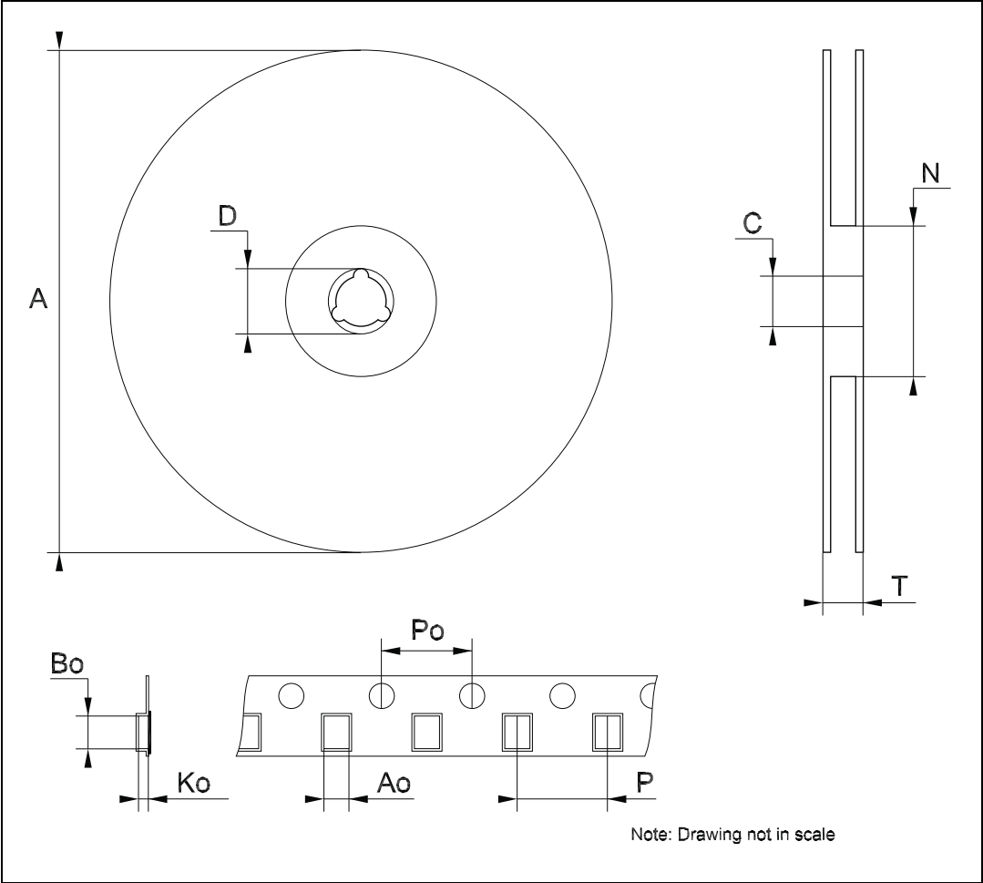
Figure 25. Power SO-8 (exposed pad) tape and reel dimensions
