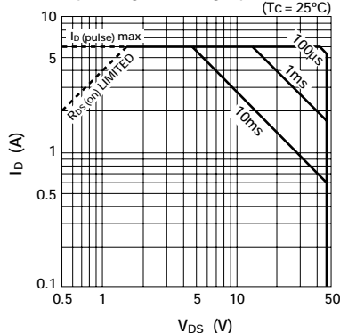
■ Safe Operating Area (single pulse) (T c = 25°C)
