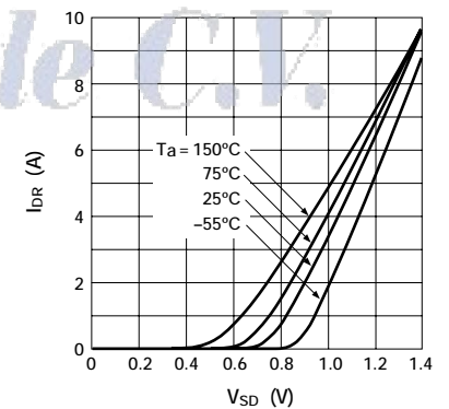
■ I DR - V SD Characteristics
