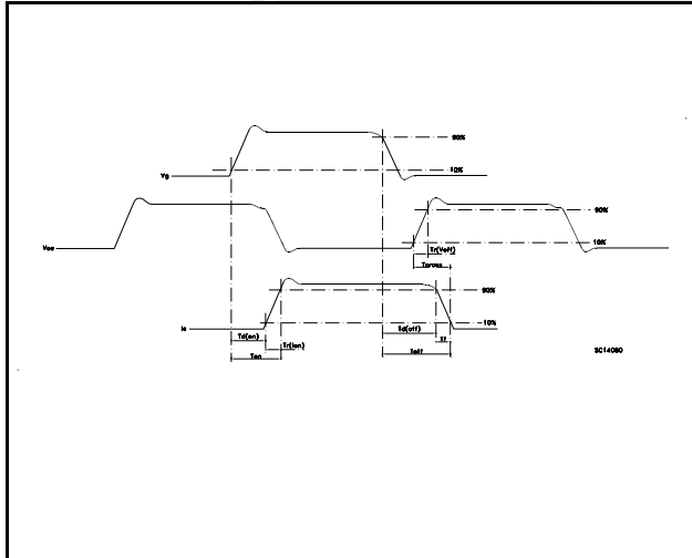
Figure 20: Switching Waveforms
