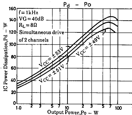
Fig.1 STK4231II Pd - Po ( R_L = 8\Omega )
