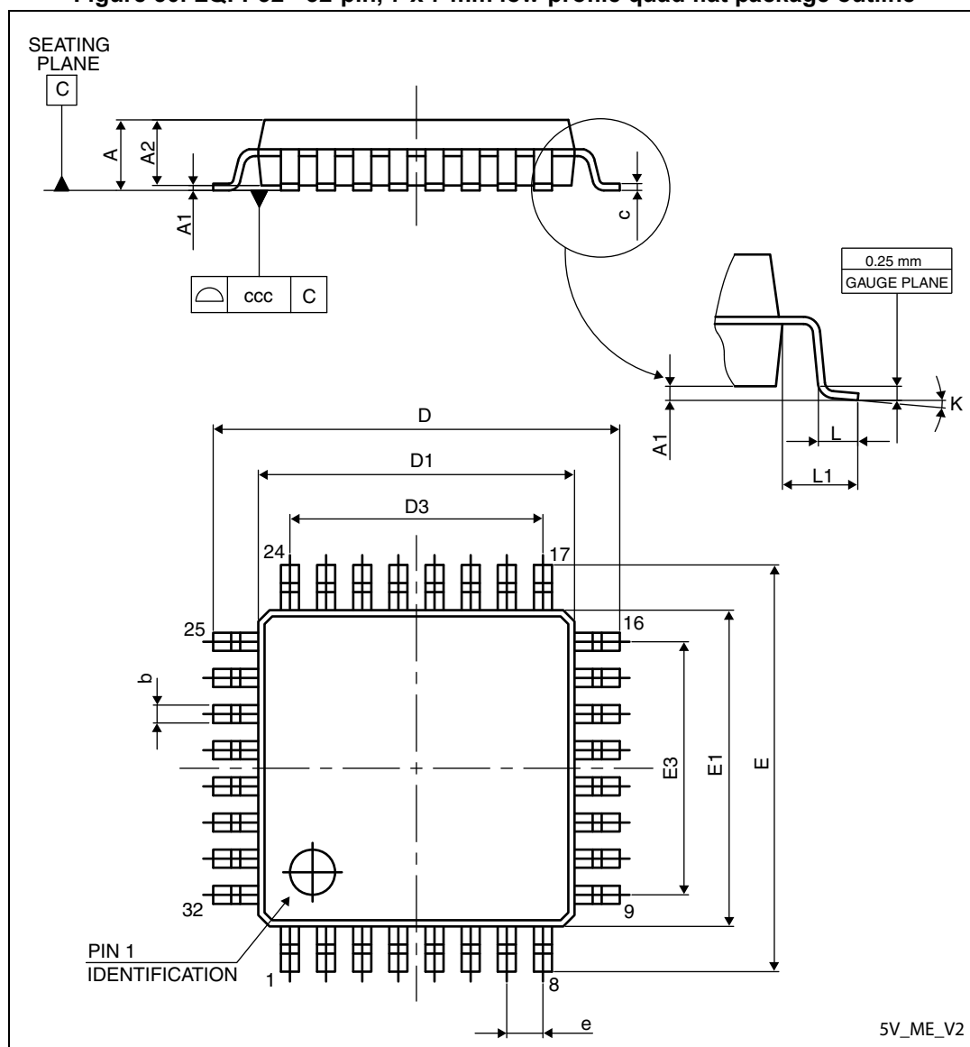
Figure 50. LQFP32 - 32-pin, 7 x 7 mm low-profile quad flat package outline
