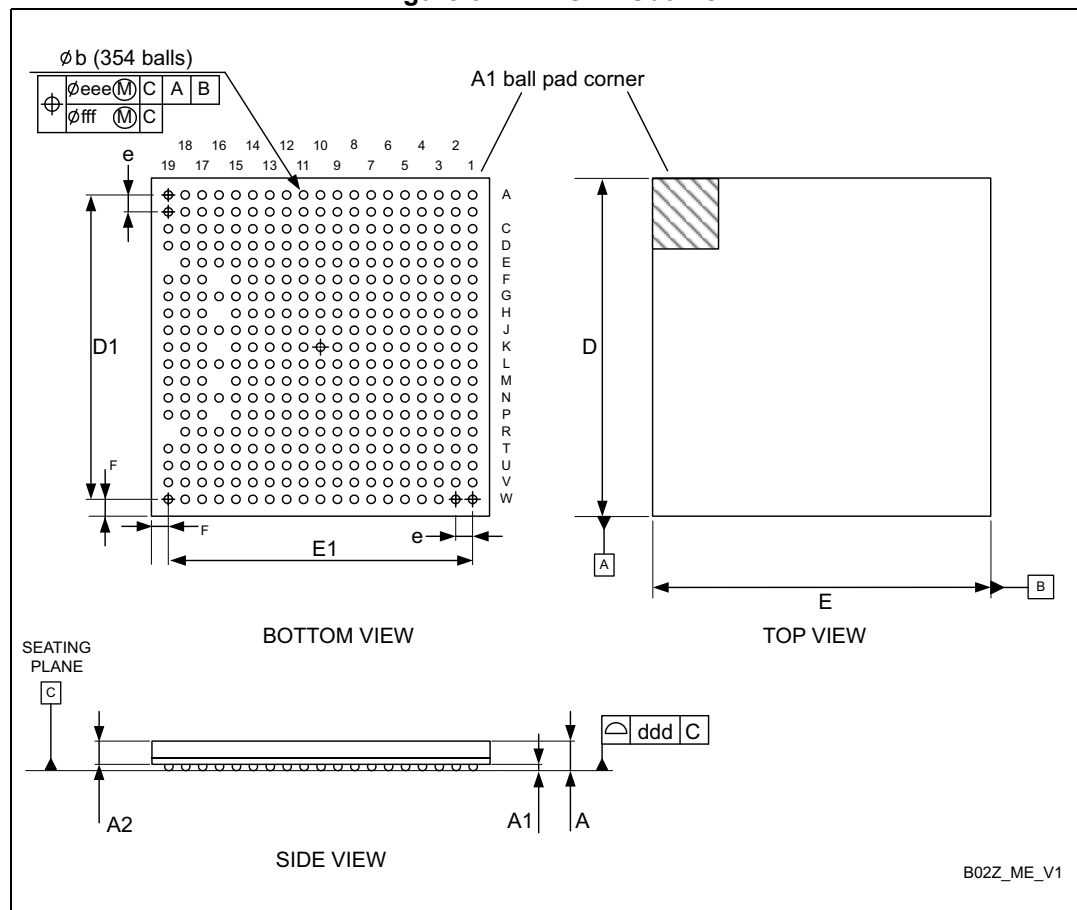
Figure 67. LFBGA - Outline
