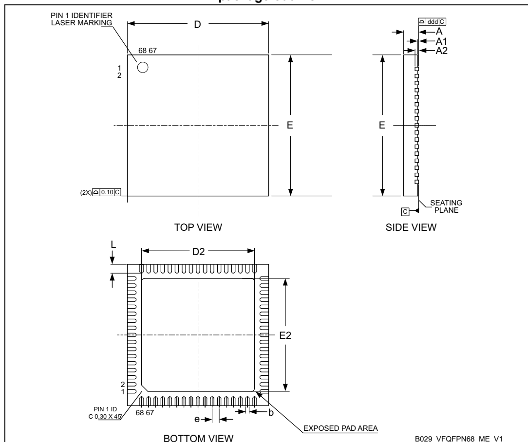
Figure 36. VFQFPN68, 8 x 8 mm, 0.4 mm pitch, very thin fine pitch quad flat package outline
