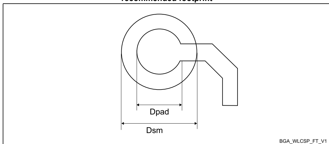
Figure 35. UFBGA - 129 balls, 7 x 7 mm, 0.5 mm fine pitch, square ball grid array recommended footprint
