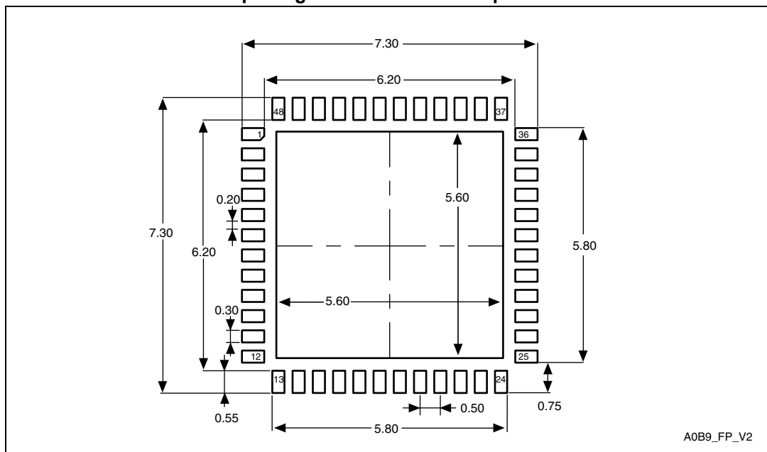
Figure 39. UFQFPN48 - 48-lead, 7 x 7 mm, 0.5 mm pitch, ultra thin fine pitch quad flat package recommended footprint
