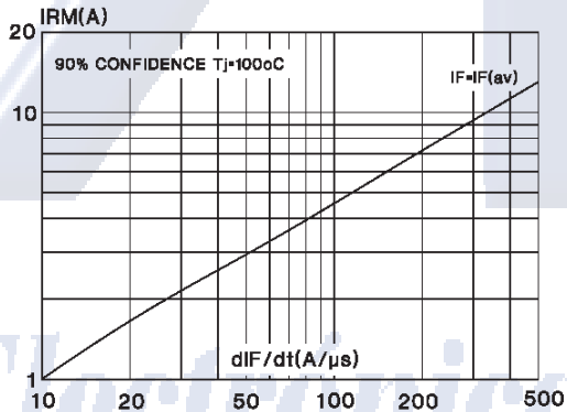
Fig. 9: Peak reverse current versus dI_F/dt (per diode).
